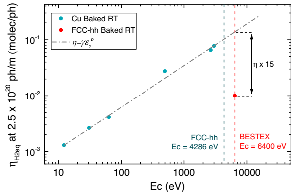
FIG. 5. Blue dots: \eta_{\text{Heq}} dependence on \varepsilon_c for RT flat Cu at a common accumulated photon dose of 2.5 \times 10^{20} ph/m as calculated from Refs. [23,27]. Dot-dashed line: fit of \eta_{\text{Heq}} as a function of \varepsilon_c for RT flat Cu according to Eq. (2). Red dot: \eta_{\text{Heq}} for FCC-hh BS at an accumulated photon dose of 2.5 \times 10^{20} ph/m.
