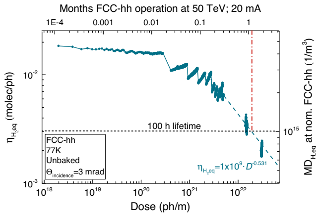
FIG. 7. Evolution of \eta_{\text{H}_2,\text{eq}} as a function of the 3 mrad glancing photon dose accumulated on the FCC-hh BS prototype at 77 K. Black horizontal dotted line represents the threshold below which the FCC-hh beam lifetime is > 100 h corresponding to a \text{H}_2 eq MD of 1 \times 10^{15} \text{ m}^{-3} . Dashed line represents the extrapolation of the data according to the observed decaying trend with the accumulated photon dose.
