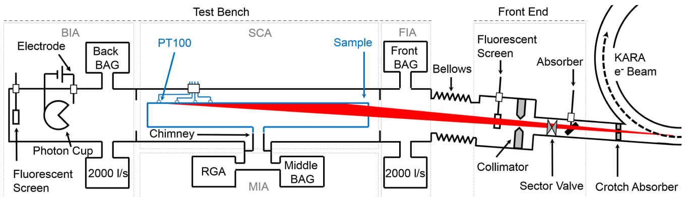
FIG. 1. Schematic layout of BESTEX [10].
