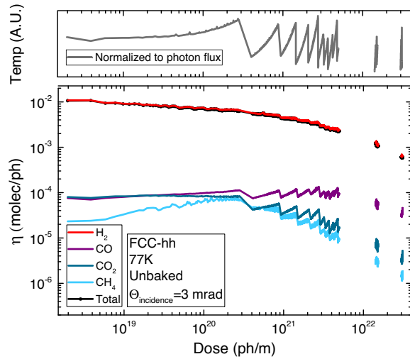
FIG. 6. Upper panel: evolution with the accumulated photon dose of the sample's temperature normalized to the absorbed photon flux. Lower panel: Evolution of \eta presented for \text{H}_2 (red line), \text{CO} (purple line), \text{CO}_2 (green line) and \text{CH}_4 (blue line) as a function of the accumulated 3 mrad photon dose accumulated on the FCC-hh BS prototype at 77 K. Black line represents the evolution of the total molecular yield obtained by summing up the contribution of each gas.
