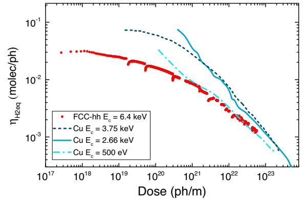
FIG. 4. H_2 equivalent molecular PSD yields ( \eta_{H_2\text{eq}} ) for baked Cu at RT as obtained from the bibliography at \epsilon_c = 3.75 keV (dashed line) [23], \epsilon_c = 2.66 keV (solid line) [26], and \epsilon_c = 500 eV (dot-dashed line) [30] compared with the measured yield for FCC-hh (red dots).
