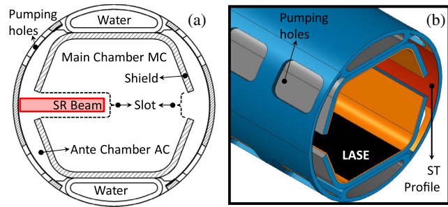
FIG. 2. Graphic descriptions of the BS design in which compliance the sample presented in this work were manufactured. (a) Cross section of BS. The red square represents the area of the SR beam. (b) 3D representation of BS in which the disposition of the sawtooth profile, LASE surface and pumping holes are visible.
