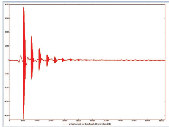
Figure 8: Snapshot of the device server of the oscilloscope used for fill pattern measurement during one of the very first injections.
