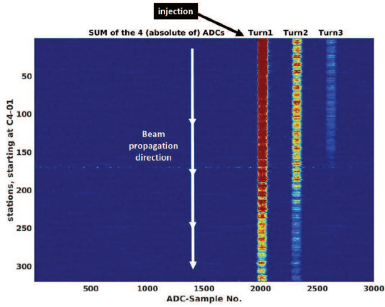
Figure 1: One of the first injection in the EBS storage ring, seen by the BPM system in ADC mode. One turn corresponds to 304 ADC samples, the beam is moving from the top to the bottom.
