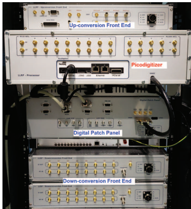
Figure 3: Rear Panel of DLLRF Setup of High Power RF lab of Sirius.
