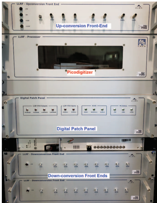
Figure 2: Front Panel of DLLRF Setup of High Power RF lab of Sirius.
