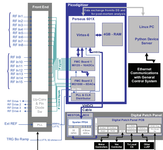
Figure 1: Main hardware components of Sirius DLLRF.
