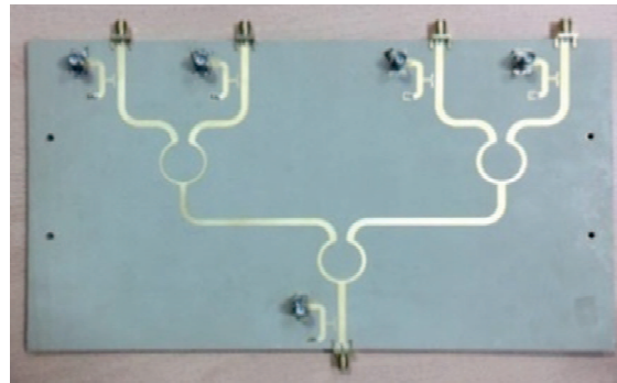
Figure 5: Power combiner with directional couplers.
