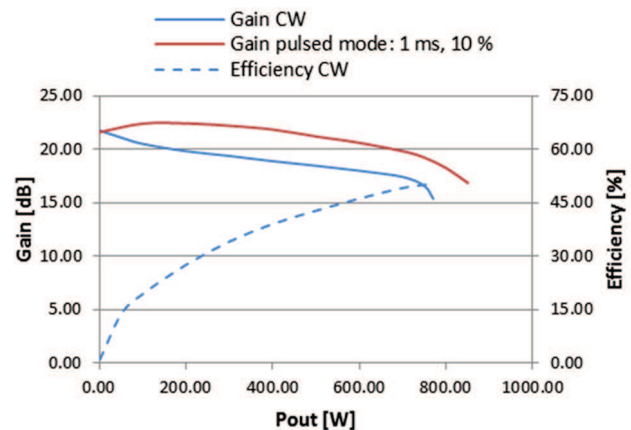
Figure 9: 1 kW power amplifier measurement results under CW and pulse mode operation.
