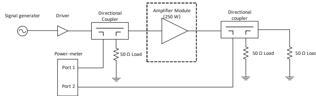
Figure 2: A 250 W amplifier module test setup.
