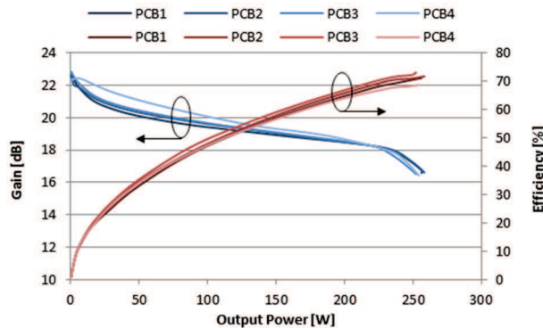
Figure 3: Four 250 W amplifier modules performance measurements.
