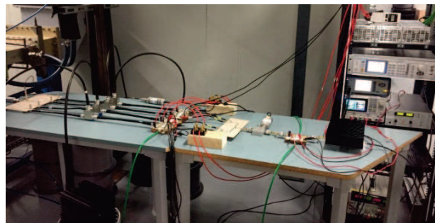
Figure 6: 1 kW SSPA test setup assembly.
