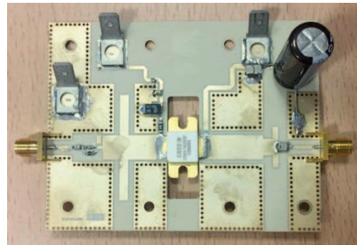
Figure 1: A 1.5 GHz power amplifier module.
