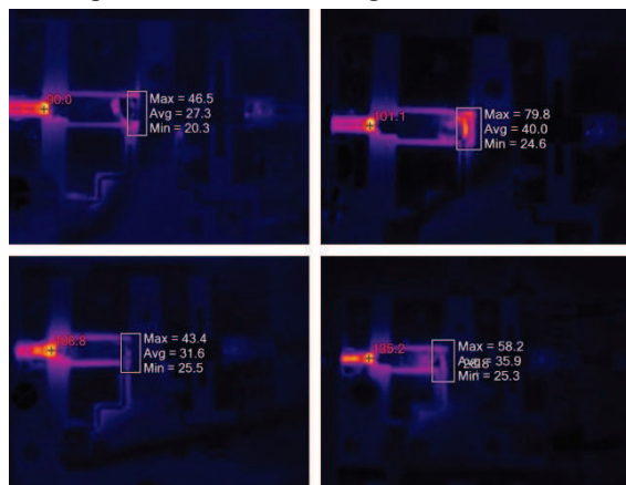
Figure 8: Thermal performance of four 250 W SSPA modules.
