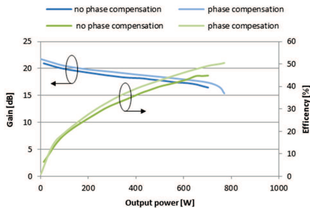
Figure 7: RF parameters measurement with and without phase compensation.
