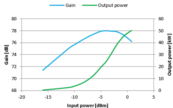
Figure 3: SSPA transmitter output power and gain.
