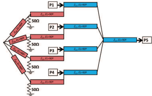
Figure 1: Gysel Combiner topology.
