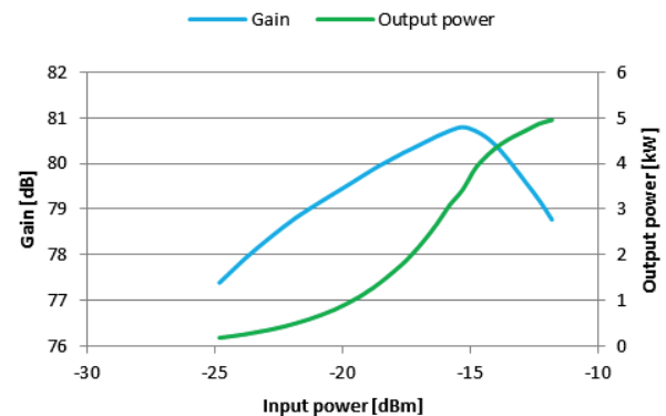
Figure 4: SSPA transmitter output power and gain.
