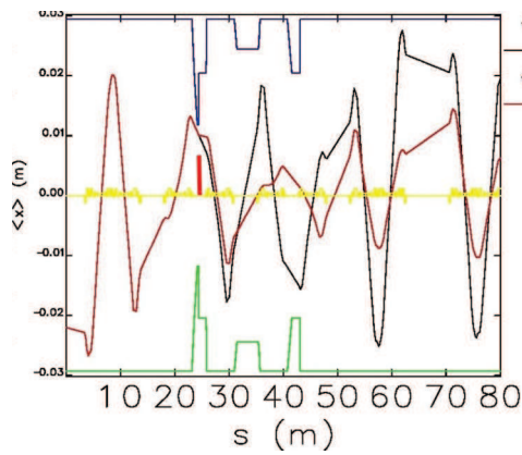
Figure 4: ELEGANT tracking for the injection with PMK placed at s = 25 m in ALBA. The amplitude of the injection trajectory and the vacuum chamber aperture from the IP are shown with the kicker off (black line) and on (red line) through the first quarter of the ring.
