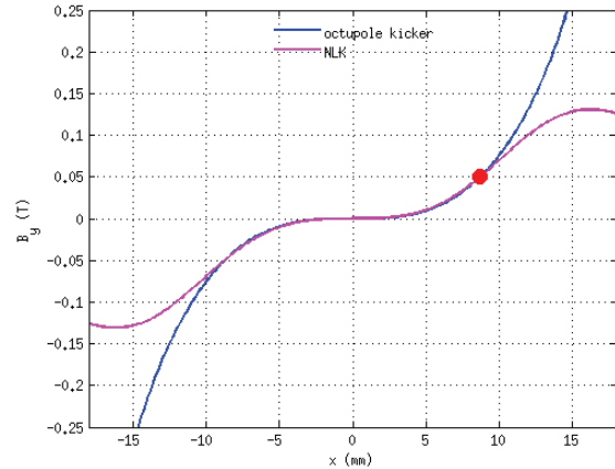
Figure 3: Magnetic field in the midplane of octupole kicker (blue line) and of NLK design (magenta line) for ALBA. The injected beam is at +8.7 mm (red circle).
