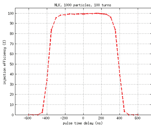
Figure 5: Capture efficiency as a function of time delay in the kicker pulse for the NLK case (lattice without errors and injection angle x'_i = -0.25 mrad).
