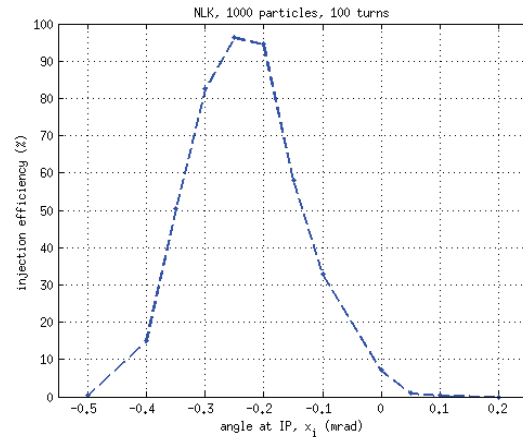
Figure 6: Capture efficiency for NLK case calculated as percentage of survived particles after 100 turns in a lattice including misalignment, orbit correction and beta-beating (average efficiency for 40 seeds). The peak of 96.5% is at x'_i = -0.25 mrad and the maximum change in the angle at IP to keep the efficiency above 75% is \pm 0.07 mrad.
