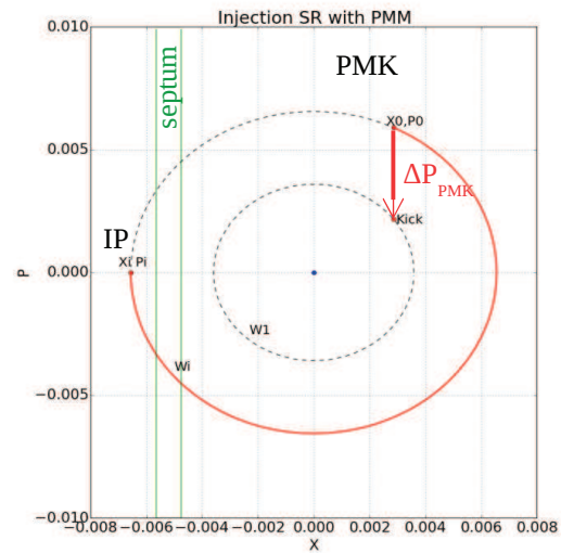
Figure 1: Injection with PMK: the beam describes a circle in the normalised phase space every phase advance of 2\pi rad. The beam is injected at the IP (septum exit) with a large invariant W_i and travels through the storage ring lattice until the point with \varphi_{PMK} = 1.68 \cdot 2\pi rad where it is kicked into the reduced invariant W_l by the PMK.
