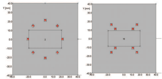
Figure 2: Geometry of the octupole kicker wires (left) and of NLK (right) for ALBA designed with OPERA-2D.
