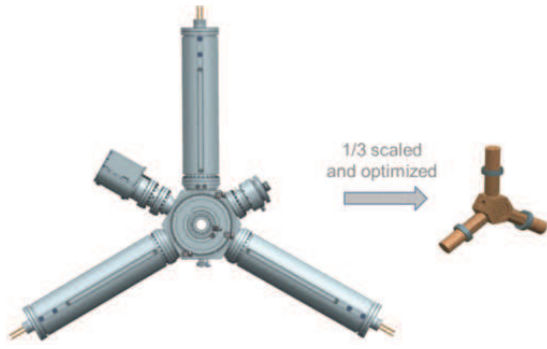
Figure 1: HOM damped cavity vs. scaled and optimized 3HC HOM cavity.
