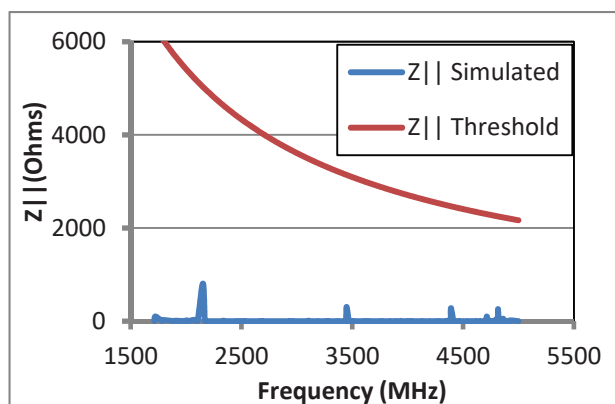
Figure 5: Simulated longitudinal impedance.
