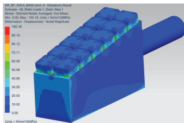
Figure 7. Absorber wedge Von Misses Stresses
