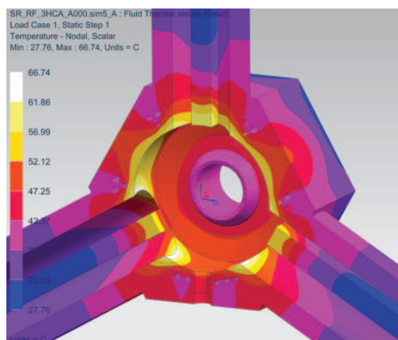
Figure 6: Cavity temperature distribution
