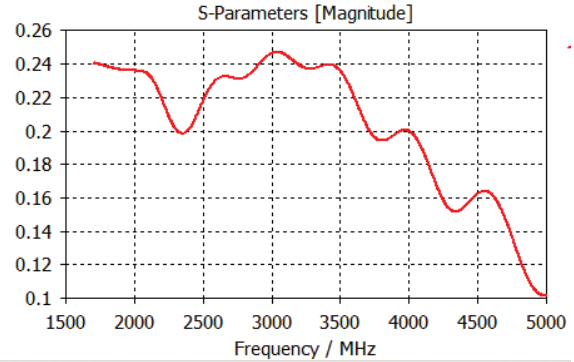
Figure 4: Reflection coefficient of the optimized damper.
