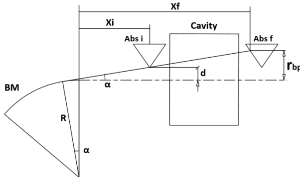
Figure 3: Raytracing schematic.
