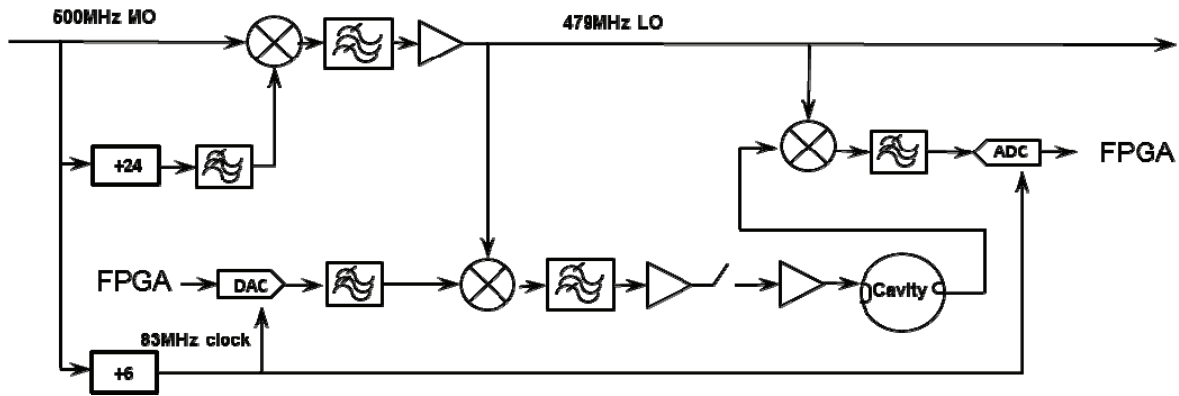
Figure 2: Schematic of RF signal processing.
