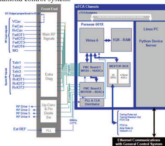
Figure 1: DLLRF block diagram.
