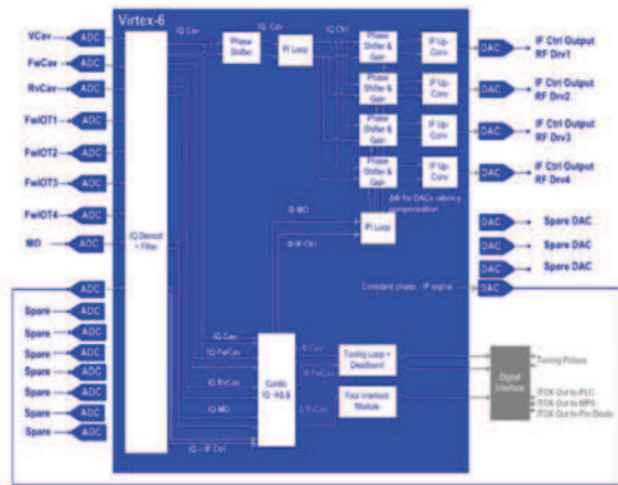
Figure 3: DLLRF firmware schematic.
