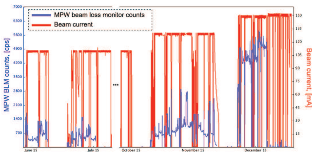
Figure 11: Beam losses measured on top of the MPW vacuum chamber throughout part of 2015, indicating a drastic dependence on beam current.
