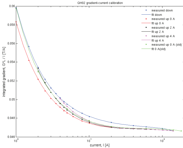
Figure 1: Calibration of the quadrupole QH02 gradient against the excitation current. The integrated gradient divided by the current, \int G(z)dz/I , is shown for different rising curves from a minimum of 0 A, 2 A and 4 A compared with the old calibration. The descending curve is common to all the cycles and is used for the quadrupole waveform definition.
