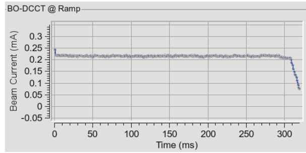
Figure 5: Measured stored current in the booster in the 67 MeV-3 GeV mode. The extraction is switched off and the beam survives in the full 320 ms long accelerating-decelerating cycle.
