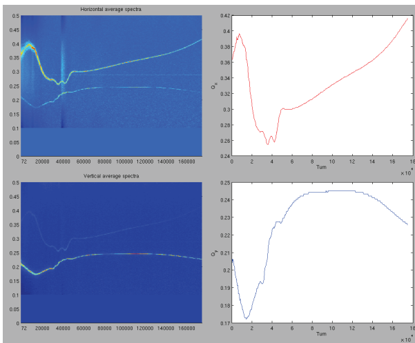
Figure 4: Measured tunes along the ramping from 67 MeV to 3 GeV. The horizontal (top) and the vertical tune (bottom) are shown against the number of turns.
