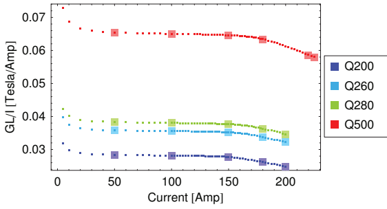
Figure 1: Integrated gradient normalized to the excitation current as a function of the current setpoint for each type of ALBA SR quadrupole. Large symbols stand for the original data provided by the manufacturer, and small symbols correspond to the detailed measurements carried out at ALBA.
