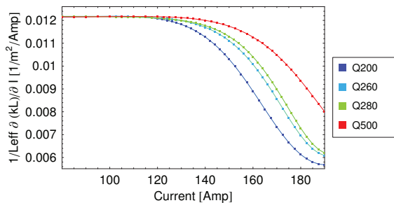
Figure 2: Slope of the quadrupole integrated strength when changing the current setting for each type of ALBA SR quadrupole. Results have been normalized by the magnet's effective length for ease of comparison.
