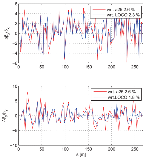
Figure 4: Beta beat measurement at the quadrupoles respect to the bare model (red lines) and respect to the model reconstructed by LOCO (blue lines). The upper plot shows the horizontal values while the lower one shows the vertical ones.
