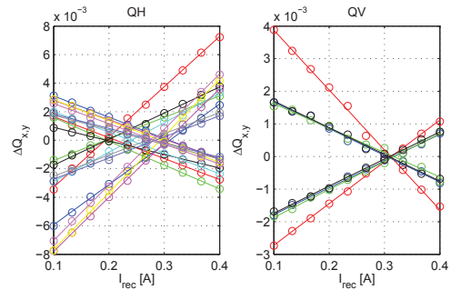
Figure 3: Tune difference with respect to the nominal as a function of the recovery current. Each family is represented in a different color. Horizontally focusing magnet families are shown in the left hand side plot while the vertical focusing ones are in the right hand side plot. The horizontal tune is represented by positive slope lines in the left hand side plot and by negative slope lines in the right hand side plot, the other way around for the vertical tune.
