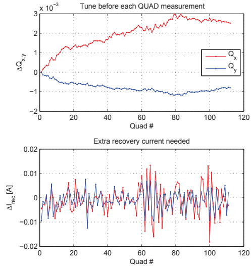
Figure 5: The upper plot shows the tune change after each magnet measurement and having applied the corresponding recovery current. The lower plot shows the corresponding additional recovery current to compensate each tune change.
