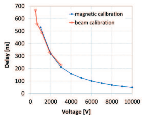
Figure 8 VER pinger magnet synchronisation
