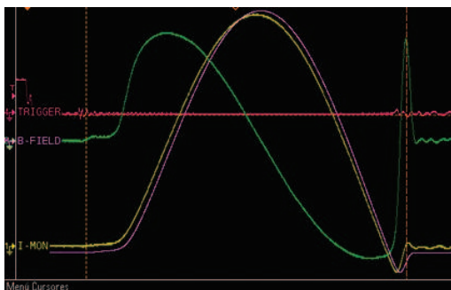
Figure 6 Image from magnetic measurements. Yellow trace is the current pulse, green is the induced voltage pulsed and purple is the integrated magnetic field
