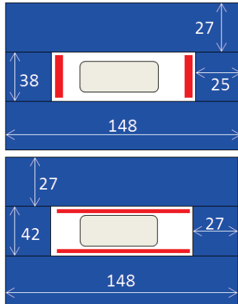
Figure 2 Cross section sketch of the HOR (upper) and VER (lower) pinger magnet. Dimensions in mm.
