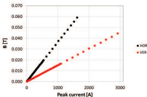
Figure 7 Magnetic field linearity with current pulse
