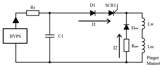
Figure 4 Schematics of the pulser unit
