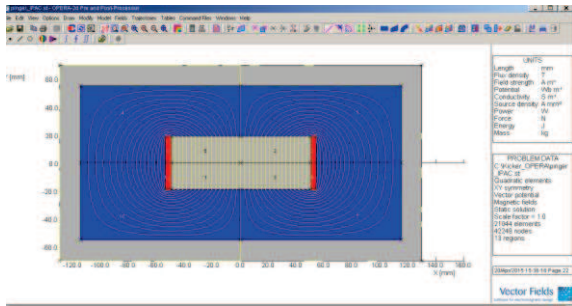
Figure 3 OPERA 2d simulation of the HOR pinger magnet
