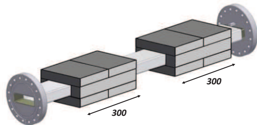
Figure 1 Installation of the magnets around the ceramic vacuum tube. Ferrite length in mm.
