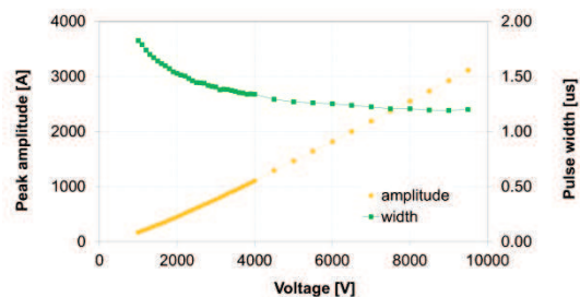
Figure 5 Peak amplitude and pulse width for the VER pinger as a function of HV setting
