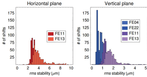
Figure 4: Stability of the photon beam position ( rms value) at the FE XBPMs calculated over periods of 8 hours.
