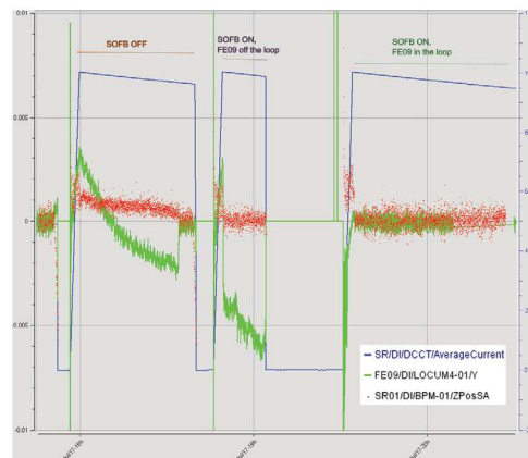
Figure 1: Comparison of photon beam motion at the XBPM of FE09-Mistral (green line) after injection with (i) SOFB off, (ii) SOFB on using only BPM data, (iii) SOFB on including the FE09-XBPM in the correction loop. Red points show as a reference the vertical position of the electron beam at a particular BPM.
