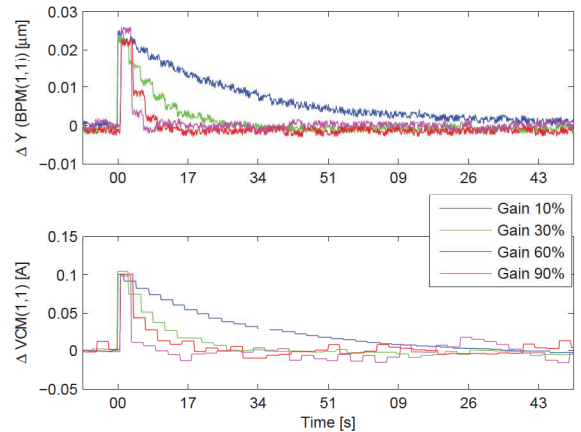
Figure 3: Response of the SOFB to a step change in the first vertical corrector. There is a small overshoot for the 90% gain.
