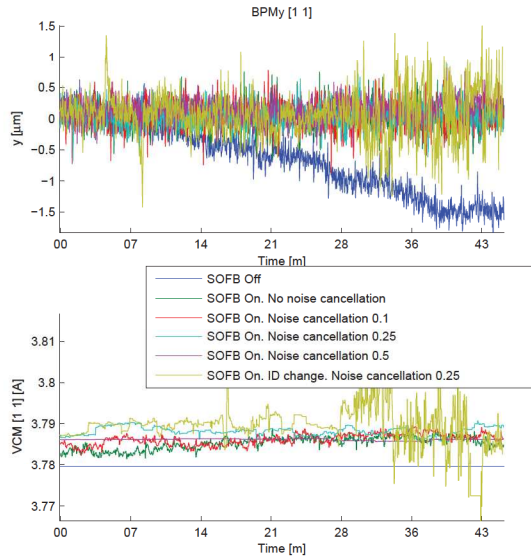
Figure 2: Noise reduction for different values of the threshold. The changes in the vertical corrector magnets (lower plot) are less frequent for higher values of the noise reduction, while the position stability (upper plot) is good in all the cases. The operational value of 0.25 is a good compromise and works well even when the ID gap are changing.
