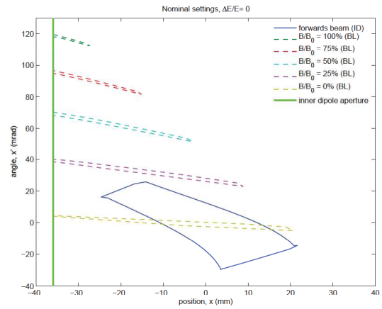
Figure 4: ID beamlines: phase space boundaries at the entrance to the bending for different degrees of dipole failure.
