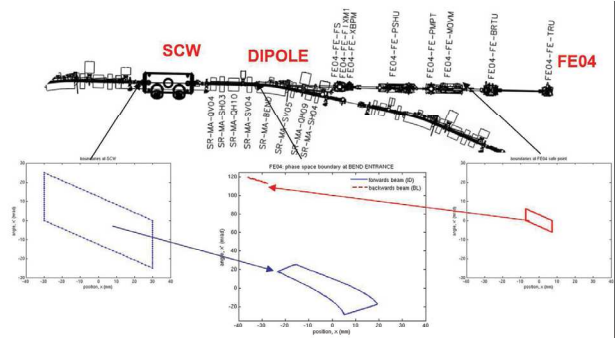
Figure 1: Section of the storage ring used for the tracking studies in the case of an ID beamline. Initial phase-space coordinates for the forwards tracked beam (bottom left), for the back tracked beam (bottom right) and final distributions (bottom centre) are shown: in this example the two distributions do not overlap, indicating a safe situation.
