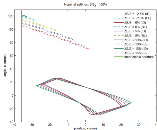
Figure 3: ID beamlines: phase space boundaries at the entrance to the bending for different degrees of energy offset.
