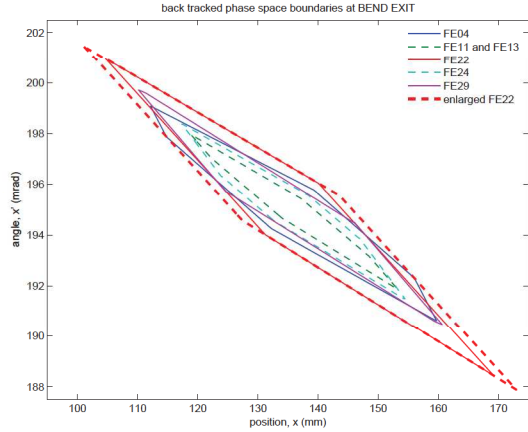
Figure 2: The phase space boundaries enclosing all possible trajectories for each of the ALBA ID beamlines compared at the dipole exit. Positions and angles are stated with respect to the stored beam centre line.
