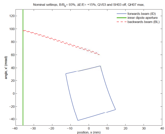
Figure 5: ID beamlines: phase space boundaries at the entrance to the bending magnet in the worst combination of errors.
