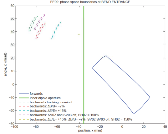
Figure 7: Dipole beamline: phase space boundaries at the entrance to the bending magnet in the worst combination of errors.
