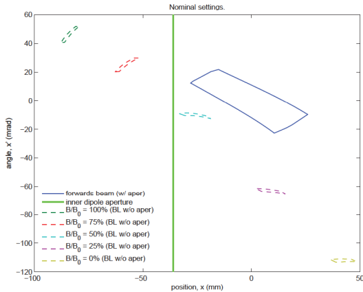
Figure 6: Dipole beamline: phase space boundaries at the entrance to the bending magnet for different degrees of dipole failure.
