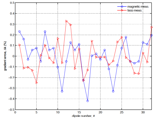
Figure 2: Comparison between the focusing strength errors \Delta k for each dipole estimated from the magnetic measurements and from the beam based measurements.
