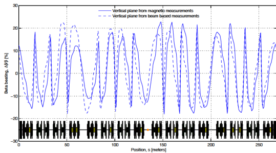
Figure 3: Vertical beta beating estimated introducing the \Delta k errors measured with the magnetic measurements and reconstructed with LOCO.
