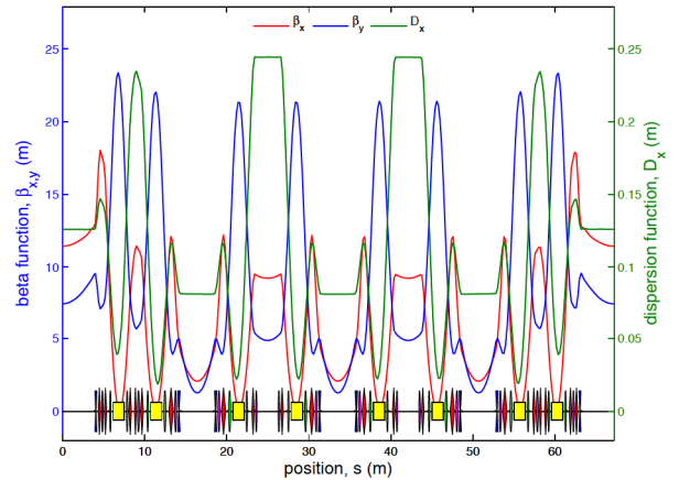
Figure 1: ALBA optical functions for one of the 4 superperiods.
